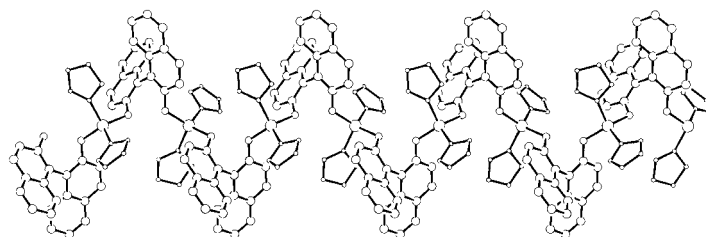
Figure 1. The [ \text{Li}\{(\text{S})\text{-Hbinol}\} ] chain of [ \text{Li}(\text{rac-Hbinol}) ] ( 2 ).
